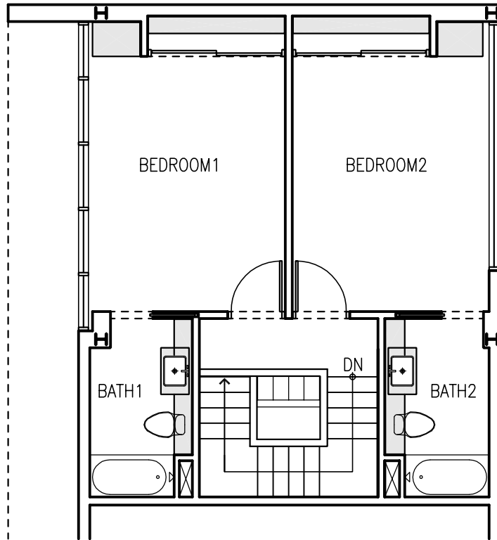
FLOOR PLAN- LEVEL 3
